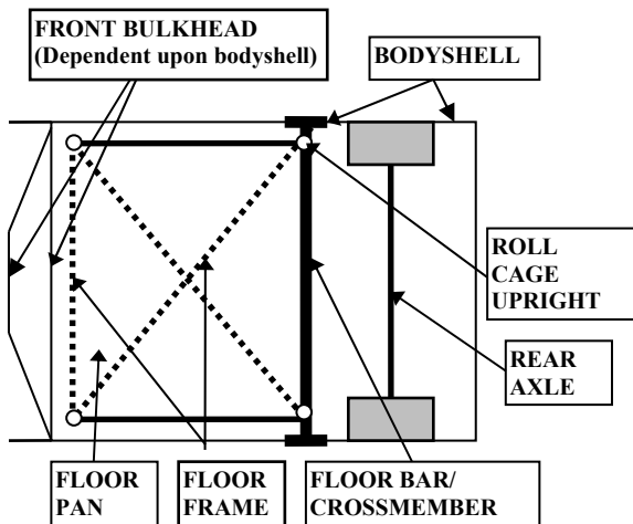
FIGURE 7 FLOOR BARS/FLOOR FRAME. Figure is diagrammatic.
