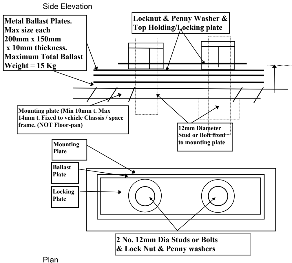
FIGURE 28 BALLAST REQUIREMENTS.
