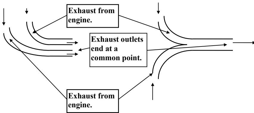
FIGURE 26b TWIN EXHAUST OUTLETS.
