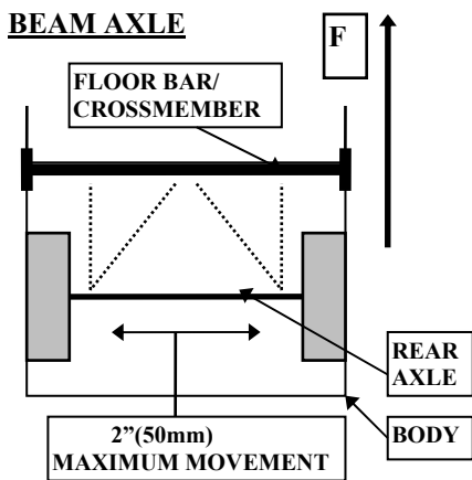
FIGURE 15 BEAM AXLE.
